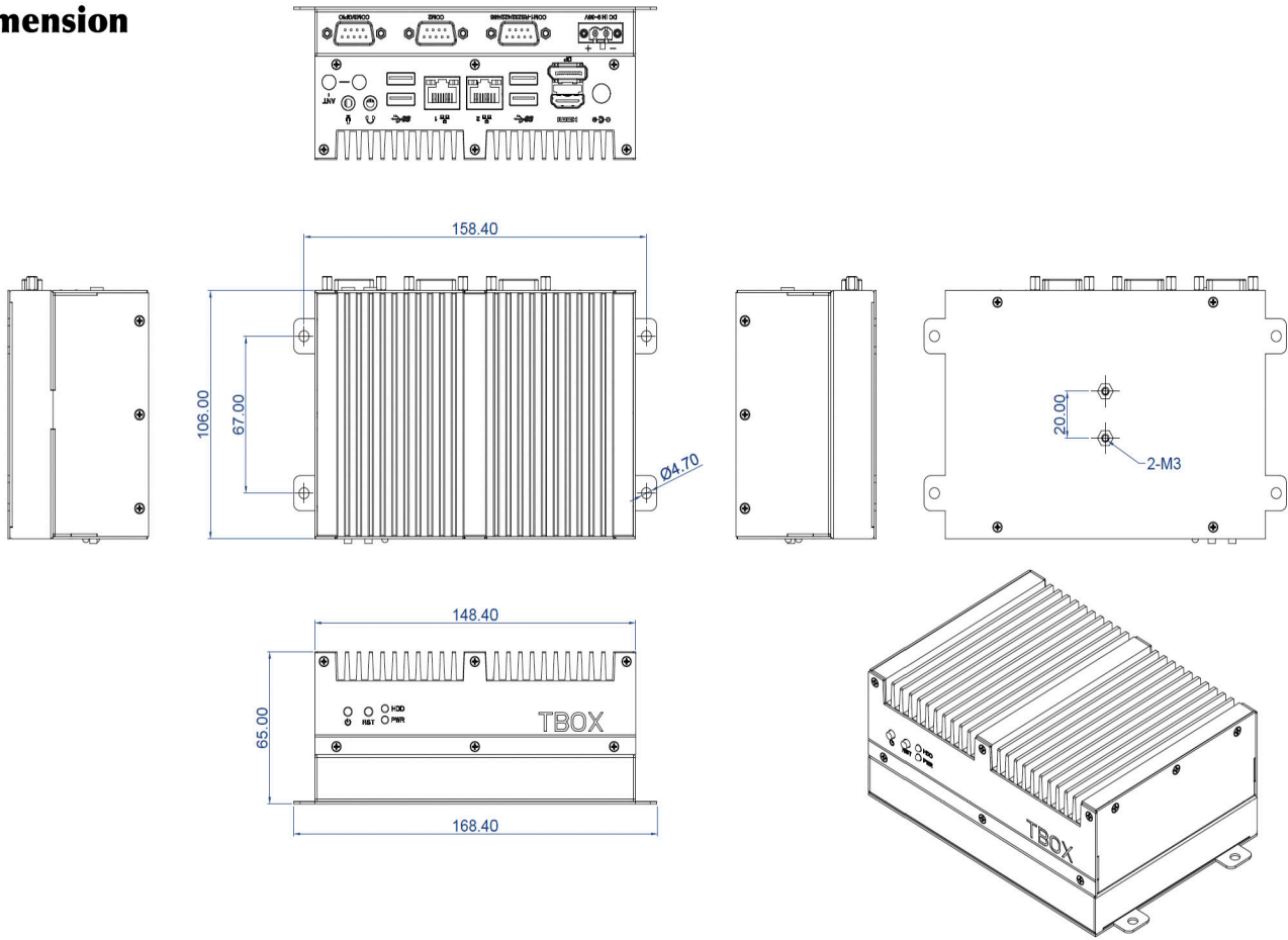
DIMENSIONAL DRAWING:TBOX-1E11
