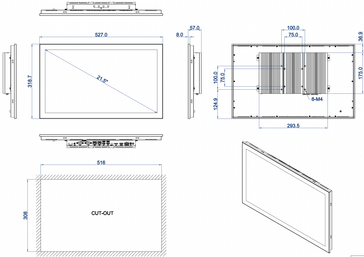
DIMENSIONAL DRAWING:TPC-DCT215
