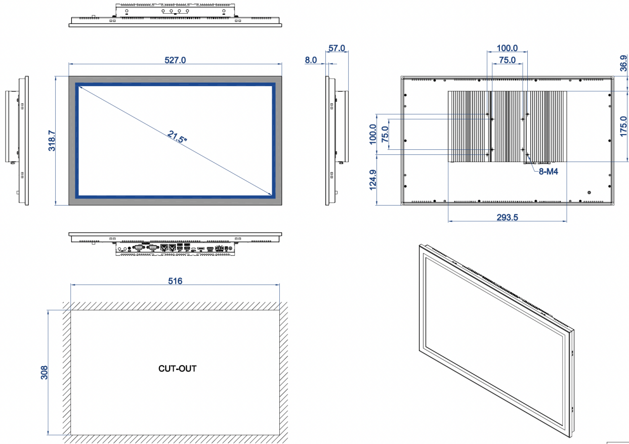
DIMENSIONAL DRAWING:TPC-DRT215
